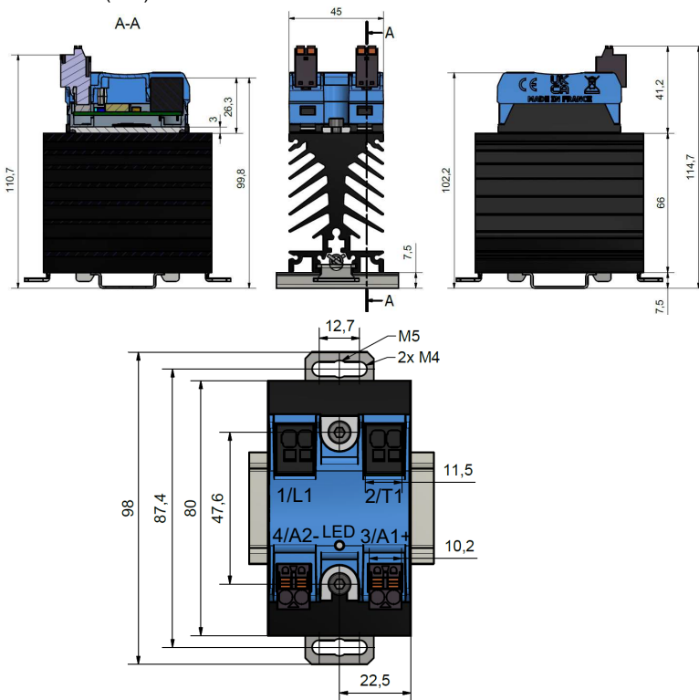
Dimensions (mm)
