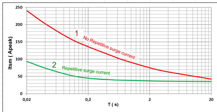
Fig.3 : Courants de surcharges / Overload currents
