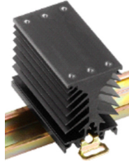
WF151100 (2-2.5 K/W)
