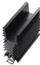
WF112xxx (0.8-1.2 K/W)
